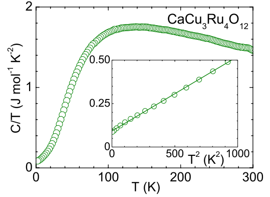
FIG. 4. (Color online) Specific heat C/T(T) of polycrystalline \text{CaCu}_3\text{Ru}_4\text{O}_{12} (main frame) and a representation C/T versus T^2 (inset). A conventional metallic Fermi-liquid behavior according to C(T) = \gamma T + \beta T^3 (solid line of the inset) is observed for T > 2 K.
