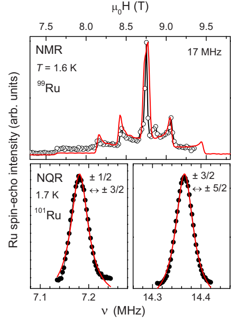
FIG. 6. (Color online) NMR and NQR spectra of polycrystalline \text{CaCu}_3\text{Ru}_4\text{O}_{12} . Upper frame: NMR spectrum of ^{99}\text{Ru} at \omega = 17 MHz and T = 1.6 K. The red solid line indicates the spectrum simulation of the quadrupolar perturbed Zeeman splitting (see text). Lower frame: NQR spectra of ^{101}\text{Ru} at 1.7 K. The red solid lines are fits with Lorentzian lines.
