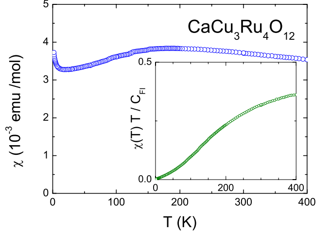
FIG. 2. (Color online) Temperature-dependent magnetic susceptibility of polycrystalline \text{CaCu}_3\text{Ru}_4\text{O}_{12} in an external field of \mu_0 H = 1 T. The inset shows \chi(T)T / C_{\text{FI}} versus T to determine the spin-fluctuation temperature T_{\text{SF}} , as described in text.
