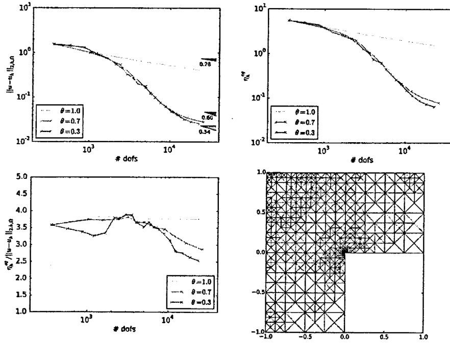
FIGURE 3. Error, estimator, effectivity index, and adaptively generated mesh ( k = 4 ).
