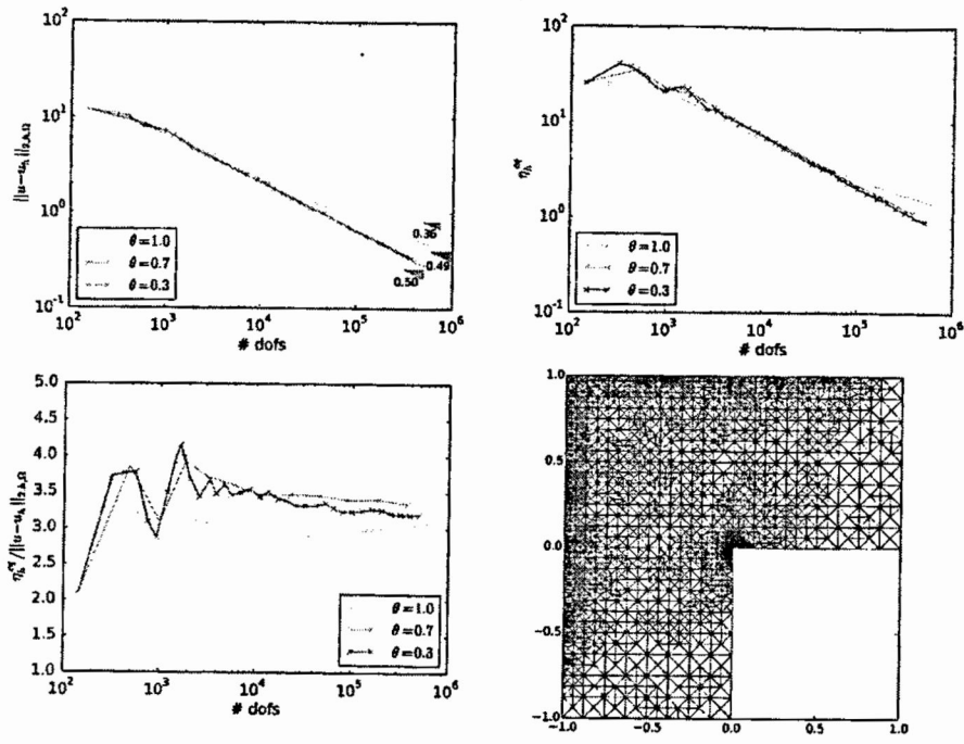
FIGURE 1. Error, estimator, effectivity index, and adaptively generated mesh ( k = 2 ).
