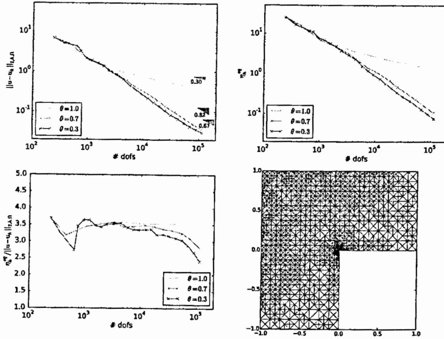
FIGURE 2. Error, estimator, effectivity index, and adaptively generated mesh ( k = 3 ).
