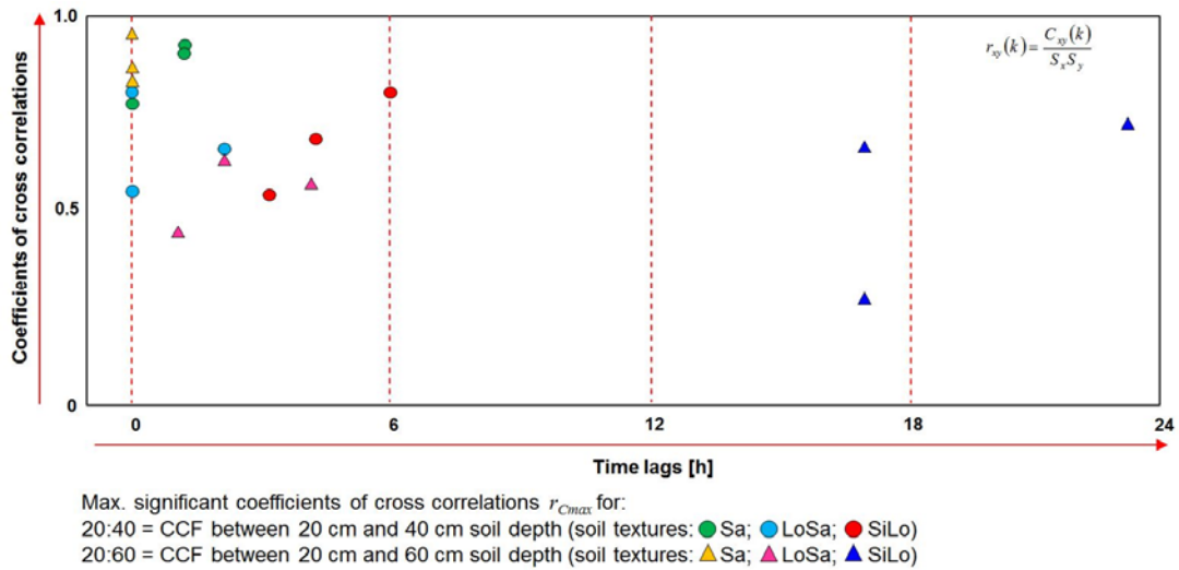
Fig. 2: Significant coefficients of cross-correlations in the 24-hour timeframe of three uniform soil profiles (significance level \alpha = 0.01 ).
