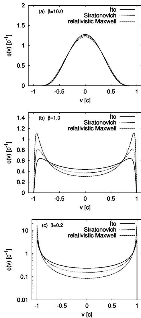
FIG. 2. Stationary solutions \phi_{\text{I/S/HK}}(v) of the relativistic Fokker-Planck equations, according to Ito (I:solid line), Stratonovich (S:dotted), and Hänggi-Klimontovich (HK:dashed-dotted). For low temperatures, i.e., for \beta \gg 1 , a Gaussian shape is approached [see (a)]. On the other hand, for very high-temperature values, corresponding to \beta \leq 1 , the distributions exhibit a bistable shape, and the quantitative deviations between \phi_{\text{I/S/HK}}(v) increase significantly as \beta \rightarrow 0 .
