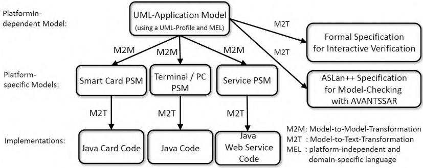
Fig. 1. SecureMDD Approach
