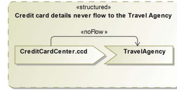
(d) Noninterference property "credit card details never flow to the TA"
