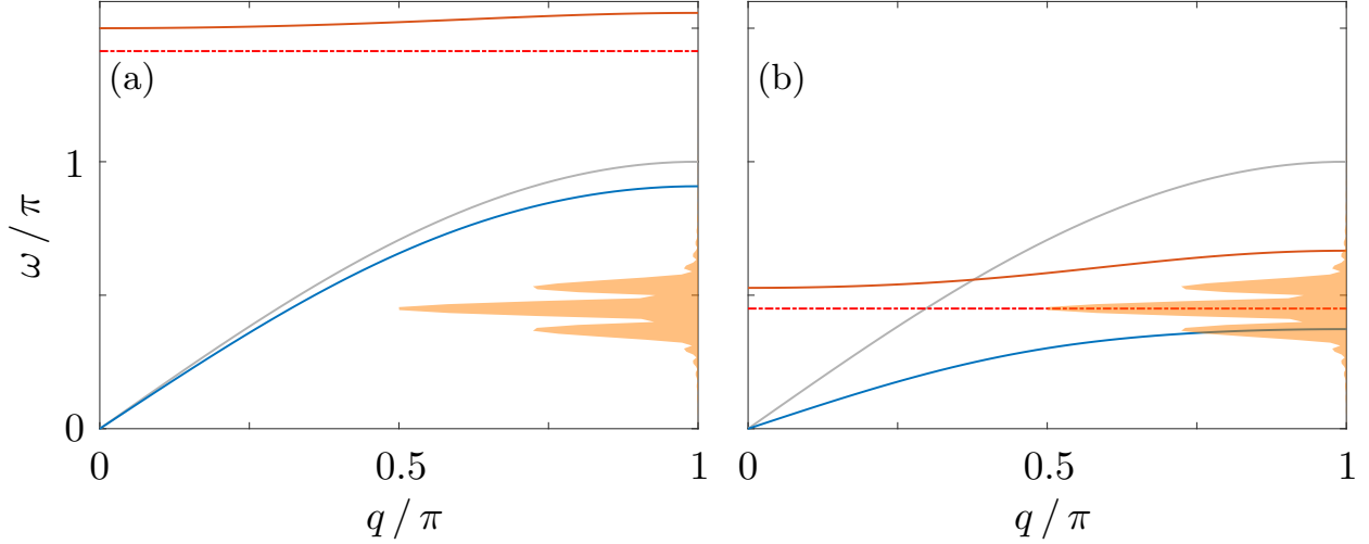
Figure 11: Band diagrams for (a) the mass-in-mass system and (b) the system with links, with m = 1 , M = m/8 and \omega_{\text{ct}} = 0.45\pi , and including the anti-resonant frequencies. The dispersion curve for the monatomic chain (—), and the Fourier transform of the toneburst forcing \mathcal{F}(F_{\text{tb}}) (■) are overlaid, where \max\{\mathcal{F}(F_{\text{tb}})\} \approx 0.006 .
