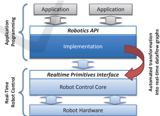
Figure 1: Robot application are programmed against the Robotics API . High-level commands specified using the Robotics API are automatically transformed into dataflow graphs at runtime and executed with real-time guarantees.
