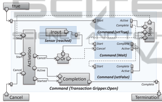
Figure 7: Transformation result for a transaction opening a gripper.
