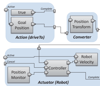
Figure 5: Transformation result for a driveTo action and a robot.
