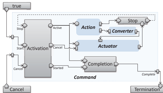
Figure 6: Transformation result for entire Platform.DriveTo command.
