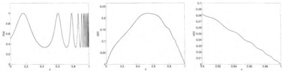
FIG. 6.2. Diffusion coefficient from (6.2) (left) and corresponding solution of (6.3) (middle) with zoom into the right end of the interval (right).
