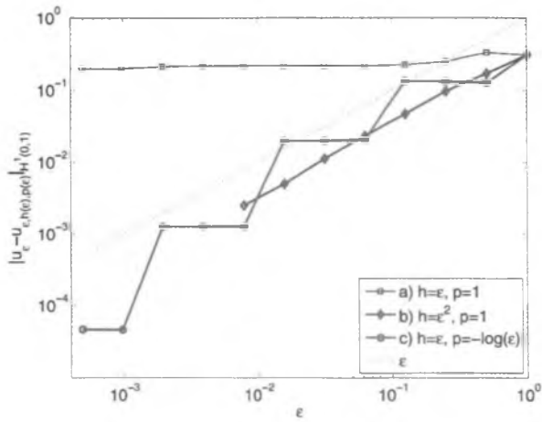
FIG. 6.1. Example from section 6.1: H^1 -error of h(\epsilon)p(\epsilon) -finite element method vs. \epsilon .
