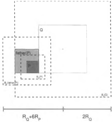
FIG. 3.2. Illustration of the proof of Proposition 3.5.
