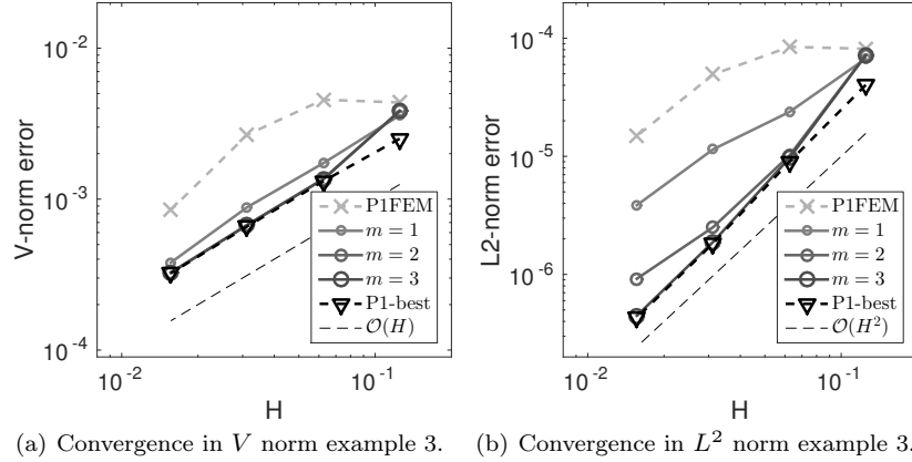
Fig. 6 Convergence history for example 3.
