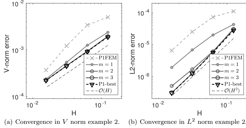
Fig. 4 Convergence history for example 2.
