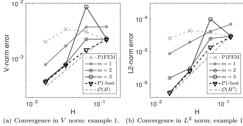
Fig. 2 Convergence history for example 1.
