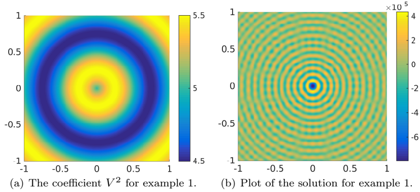
Fig. 1 Plots for example 1.
