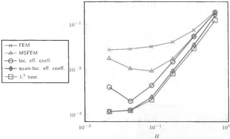
FIG. 4. Convergence history under uniform mesh refinement.
