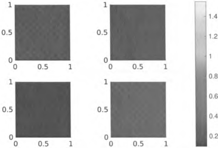
FIG. 3. Matrix entries of the reconstructed localized coefficient (A_H^{(l)}) in the first experiment for H = \sqrt{2} \times 2^{-6} .
