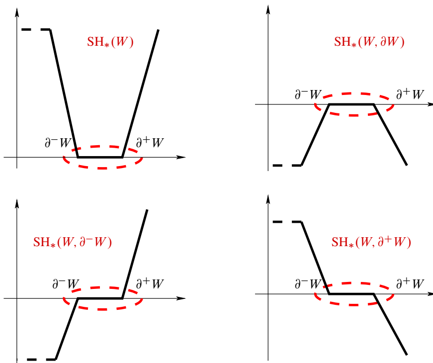
Figure 9: Shape of Hamiltonians for \mathrm{SH}_*(W, A) with A = \emptyset, \partial W, \partial^-W, \partial^+W
