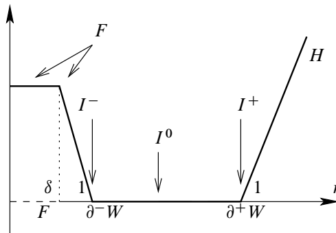
Figure 8: Cofinal family of Hamiltonians for \mathrm{SH}_*^{\heartsuit}(W)
