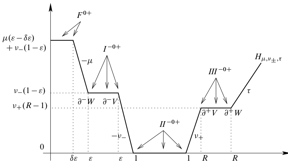
Figure 18: Hamiltonian adapted to the construction of the transfer map \mathrm{SH}_*^{\heartsuit}(W) \rightarrow \mathrm{SH}_*^{\heartsuit}(V)
