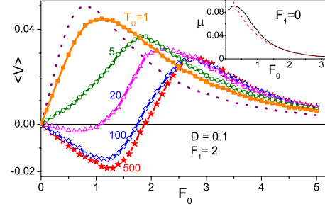
FIG. 2. (Color online) ANM for a driven-pulsated elongated Brownian particle: current \langle v \rangle vs static bias F_0 in the presence of square-wave drives with amplitude F_1=2 and different periods T_\Omega (see legend). Other simulation parameters: Diffusion strengths D=D_r=D_\phi=0.1 ; shape parameters a=0.05 , b=0.3 ; compartment parameters x_L=y_L=1 , and \Delta=0.1 . Each data point for \langle v \rangle \equiv \lim_{t \rightarrow \infty} \langle x(t) - x(0) \rangle / t was computed from a single trajectory with t=10^6 and time-step 10^{-5} ; the statistical error was estimated to be 5%, i.e., of the order of the symbol size. Note, for a comparison, that the compartment traversal time is \tau_0=7 and the diffusive relaxation times are \tau_D^{(x)} = \tau_D^{(y)} = 5 . The dotted curve represents v(F) at zero ac-drive, F_1=0 . Inset: the corresponding mobility curve (solid curve), \mu(F) , is compared with the analytical estimate of Eq. (4) (dashed curve) for F_m=0.86 .
