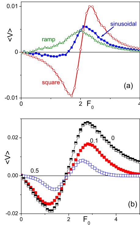
FIG. 3. (Color online) (a) Drive waveform dependence: \langle v \rangle vs F_0 for three waveforms of F_{ac}(t) , square (as in Fig. 2), sinusoidal and ramped, all with F_1=2 , D=0.02 , and T_\Omega=10^3 . (b) Particle inertia dependence: \langle v \rangle vs F_0 for three values of m=I , see text. Other simulation parameters are F_1=2 , D=0.1 , and T_\Omega=500 .
