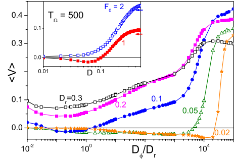
FIG. 5. (Color online) Rotational translational diffusion dependence: \langle v \rangle vs D_\phi/D_r for different values of D_r (see legend). Inset: \langle v \rangle vs D=D_r=D_\phi with D_\phi/D_r=1 . The arrows mark the asymptotes predicted in the text. Other simulation parameters are as in Fig. 4 with b=0.3 .
