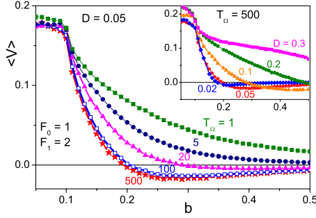
FIG. 4. (Color online) Particle elongation dependence: \langle v \rangle vs b for different values of T_\Omega (main panel) and of D (inset). Other simulation parameters: square-wave ac-drive with amplitude strength F_1=2 , and bias F_0=1 , a=0.05 , x_L=y_L=1 , and \Delta=0.1 .
