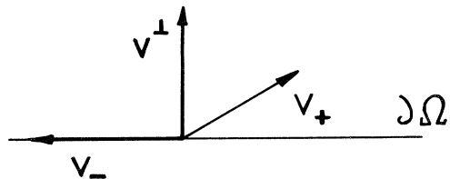
FIG. 2. Form of the local separatrix around the saddle point (\hat{a}_2, \hat{\varphi}) with corresponding eigenvectors introduced in the text.
