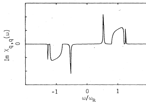
FIG. 3. The imaginary part of the frequency-dependence susceptibility, for a non-Ohmic heat bath. We exhibit the case where \omega_0/\omega_B = 0.9 , \Gamma/\omega_B = 9 , and \omega_D/\omega_B = 0.2 .
