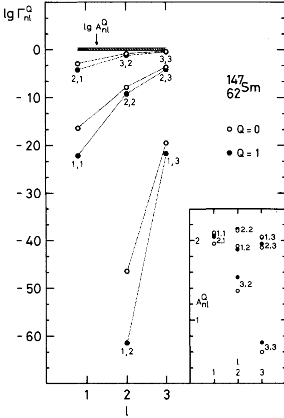
Fig. 3. Resonance widths (in MeV) for ^{147}_{62}\text{Sm} without monopole, (O), and with monopole, (●). The prefactor varies weakly within the hatched region. The inset exhibits the more detailed behaviour of this prefactor.
