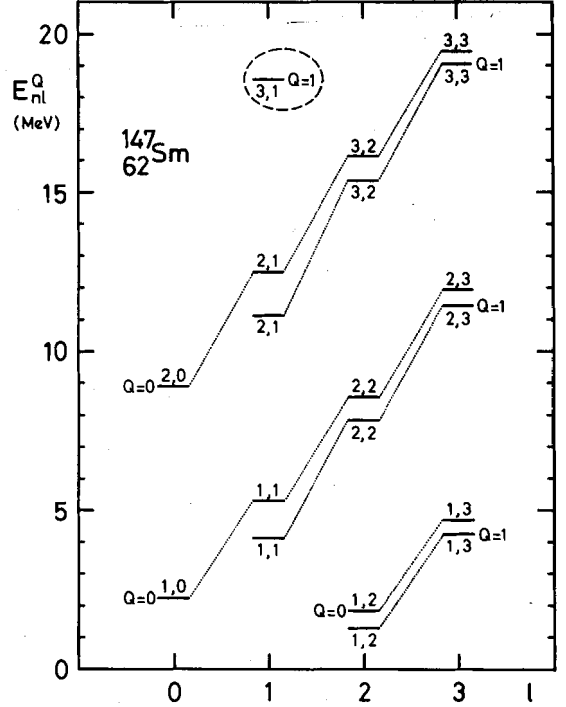
Fig. 2. Schematic alpha-particle resonance levels in ^{147}_{62}\text{Sm} for various angular momentum values l , without monopole, Q = 0 , and, correspondingly, with monopole, Q = 1 . With a monopole, there occurs a new resonance level, indicated by the enclosed, dashed ellipse.
