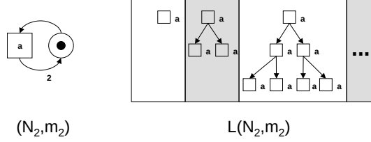
Fig. 3. Partial language without term-based representation.
