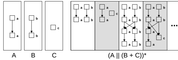
Fig. 1. Partial language given by a term.
