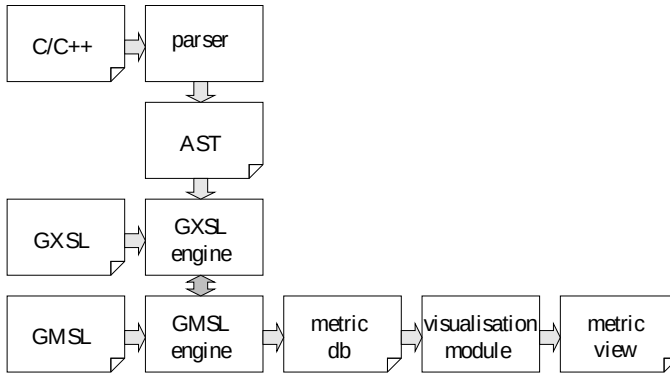
Fig. 2. GOANNA’s architecture for metric computation
