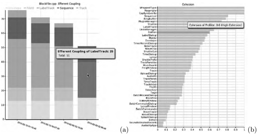
Fig. 3. (a) Histogram implementation of the time view. The histogram shows the effort coupling over time for different classes. (b) Bar chart implementation of the metric view. Ranking of classes by cohesion.
