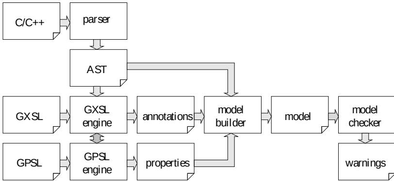
Fig. 1. GOANNA’s model checking approach for statically analyzing C/C++ code
