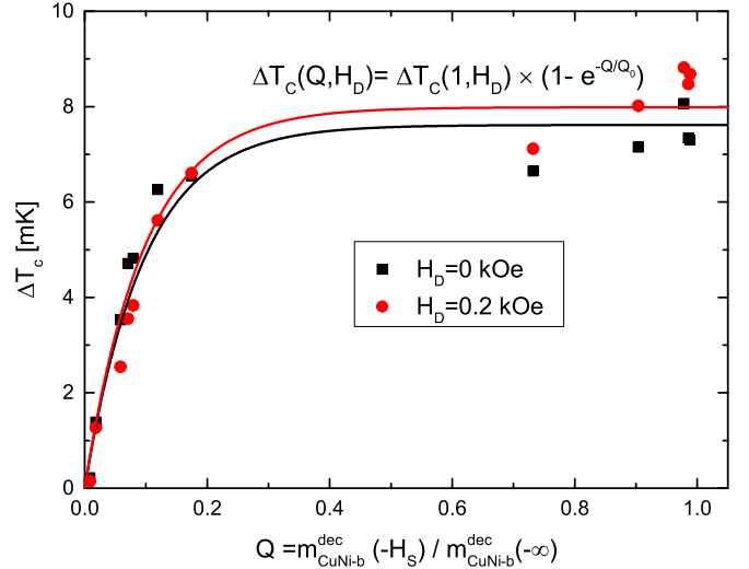
FIG. 6. Triplet SSV effect, \Delta T_c , as a function of the fraction of magnetic moment in the minor magnetic transition, turned at the negative reversal field, -H_S . The solid lines give an empirical exponential fit to the data according to Eq. (3). For details and the obtained fit parameters, see the text.
