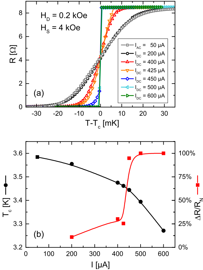
FIG. 9. (a) Superconducting transitions at H_D = 0.2 kOe and H_S = 4 kOe and various transport currents, I , plotted as a function of the temperature relative to the transition temperature, T_c . All transitions plotted have been recorded after increasing the applied field from -H_S to H_D and at decreasing T . There is an obvious sharpening of the transition above I_{DC} = 200 \mu A , yielding a transition width of less than 1 mK for I_{DC} = 600 \mu A . (b) Corresponding superconducting transition temperature (left scale, black symbols and line) and switching capability, \Delta R/R_N (for a definition, see the text), normalized to the normal state resistance (right scale, red symbols and line) as a function of the applied current. Please note that the point at I = 50 \mu A (black square) is obtained using ac current, while all other data points are obtained by measurements with dc current. The solid lines are guides to the eye.
