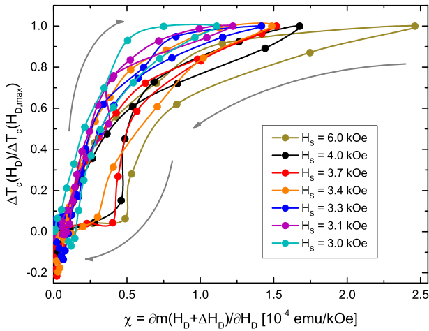
FIG. 13. Superconducting spin-valve effect, \Delta T_c(H_D) , normalized to the maximum value \Delta T_c(H_{D,\max}) for the respective H_S , as a function of the field derivative \chi = \frac{\partial m(H_D + \Delta H_D)}{\partial H_D} for increasing H_D . Here, \Delta H_D is the field shift between the maximum of the derivative and the maximum of the effect. The arrows indicate the sequence of data points from negative H_D to positive H_D (starting at zero \chi ). Solid lines are guide to the eye.
