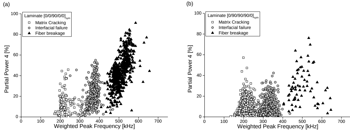
Figure 2. Representative results for the identified natural clusters for two specimens with different laminate configurations.
