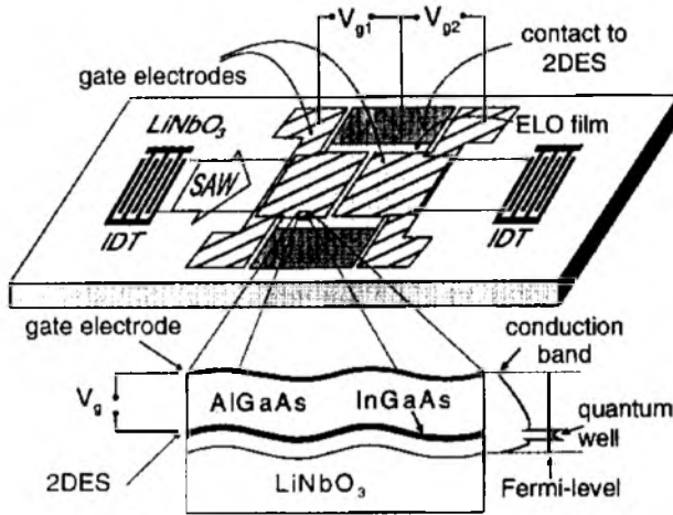
Fig. 1. Schematic sketch of the hybrid device with two gates on top of the ELO film. The thickness of the ELO film is 0.5 \mu\text{m} and the distance between \text{LiNbO}_3 and 2DES is just 32 \text{ nm} .
