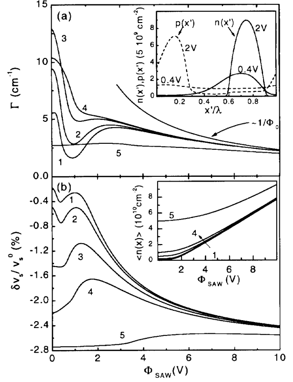
Fig. 1. The calculated absorption coefficient (a) and shift of the SAW-velocity (b) due to an electron-hole plasma as a function of the SAW potential amplitude \Phi_{SAW} for various optical excitation powers. The numbers 1-5 correspond to the photogenerated 2D carrier densities in the absence of a SAW n_{s0} = 10^9 , 2 \cdot 10^9 , 5 \cdot 10^9 , 10^{10} , and 5 \cdot 10^{10} cm -2 , respectively. \lambda = 60 \mu m; the electron mobility \mu_e = 2000 cm 2 /Vs and the hole mobility \mu_h = \mu_e/6 . The inset in (a) illustrates the separation of electron and holes into stripes with increasing SAW potential. The inset of (b) shows the average density N_e(\Phi_{SAW}) for various n_{s0} . K_{eff}^2 = 0.056 .
