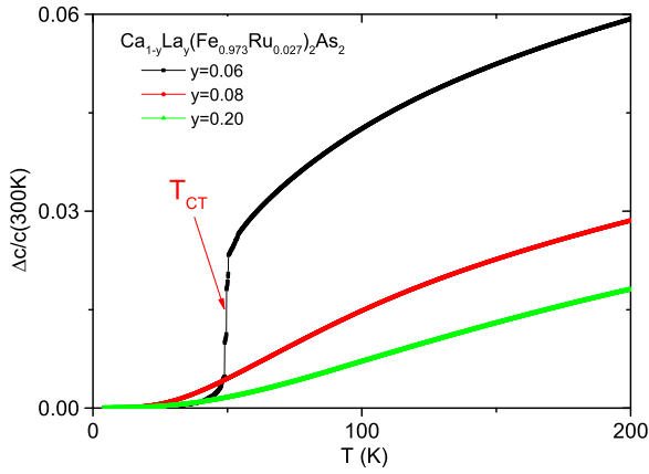
FIG. 7. (Color online) Temperature-dependent c -axis relative length change [\Delta c/c(300\text{ K}) = [c(T) - c(300\text{ K})]/c(300\text{ K})] for single-crystalline \text{Ca}_{1-y}\text{La}_y(\text{Fe}_{0.973}\text{Ru}_{0.027})_2\text{As}_2 for y = 0.06, 0.08 , and 0.20 . All data are obtained upon increasing temperature.
