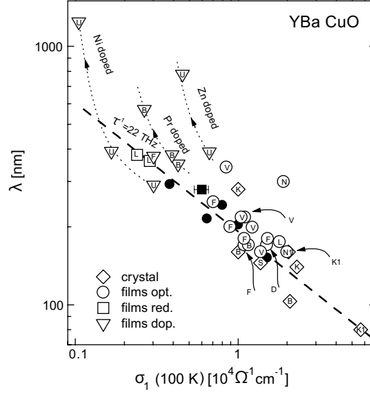
Fig. 1. – Low-temperature ( T \lesssim 10 K) penetration depth \lambda of different YBCO samples as a function of the normal-state conductivity \sigma_n at T=100 K. The dashed line is drawn according to the expression \lambda(0)^{-2}/\mu_0 = \sigma_n/\tau using 1/\tau = 22 THz. The characters in the symbols correspond to: Rhombs: single-crystal data: B Basov et al. [18] and Zhang et al. [19]; K Kitano et al. [20]; K1 Kamal et al. [22]; S Sonier et al. [21]. Circles: optimally doped \text{YBa}_2\text{Cu}_3\text{O}_{7-\delta} films: filled circles, this work, table I; B Brorson et al. [9]; D Dähne et al. [13]; F Fiory et al. [16]; L Ludwig et al. [11]; N Nagashima et al. [12] ( \lambda is taken at T = 40 K); N1 Nuss et al. [14]; V de Vaulchier et al. [15]. Squares: oxygen-reduced \text{YBa}_2\text{Cu}_3\text{O}_{7-\delta} films: filled squares, this work, table I; L Ludwig et al. [11]. Downtriangles: doped \text{YBa}_2\text{Cu}_3\text{O}_{7-\delta} films: B Brorson et al. [9] (20%, 30%, and 40% Pr-doped films); F Feenstra et al. [10] ( \text{DyBa}_2\text{Cu}_3\text{O}_{7-\delta} ); U Ulm et al. [17] (2%, 4% and 6% Ni-doped and 2% and 4% Zn-doped films). The dotted lines are guide to the eye. The arrows indicate the increasing doping direction.
