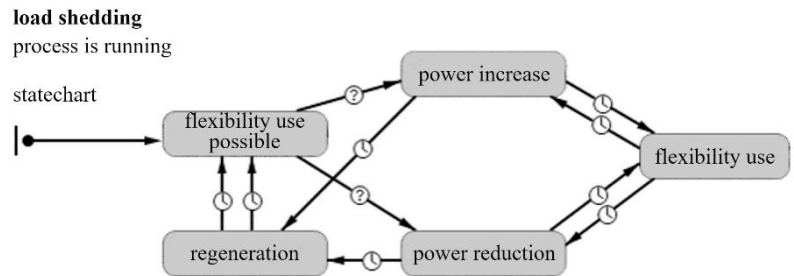
Figure 2: Flexibility statechart
