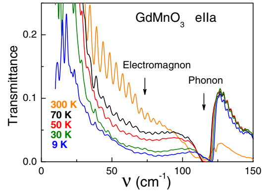
Fig. 1. (Color online) Transmittance spectra of a thin \text{GdMnO}_3 sample in the far-infrared frequency range and at different temperatures as indicated. Arrows show the position of the high-frequency electromagnon and of the lowest infrared phonon. The low-frequency electromagnon (around 23 \text{cm}^{-1} ) is not seen in this presentation.
