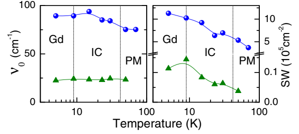
Fig. 3. (Color online) Parameters of the electromagnons in \text{GdMnO}_3 . Left panel – eigenfrequencies, right panel – spectral weight 1 (note change in scale in the vertical axis). Symbols – experimental data, lines are to guide the eye. Thin dashed lines indicate phase boundaries between different magnetic states [20,25]: PM – paramagnetic, IC – incommensurate, Gd – Gadolinium ordering. Note that in present experiments the canted magnetic state is avoided because of zero external magnetic field [9,25].
