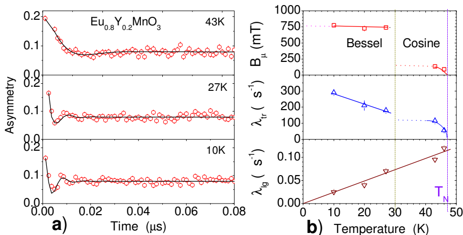
Figure 3. a): Selected ZF spectra of \text{Eu}_{0.8}\text{Y}_{0.2}\text{MnO}_3 at different temperatures. The lines are fits discussed in text. b): Temperature dependences of the local field B_\mu , the transverse ( \lambda_{\text{tr}} ) and longitudinal ( \lambda_{\text{lg}} ) relaxation rates. The lines through the data points are guides to the eye.
