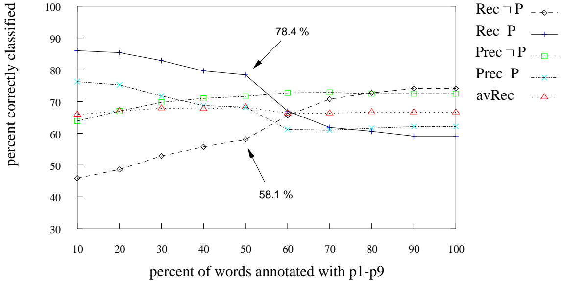
Figure 3: Prosodic classification: whole turns (TE) and S4, S3, and S2 boundaries: 4469 \supset P, 5014 P, at the 50% threshold
