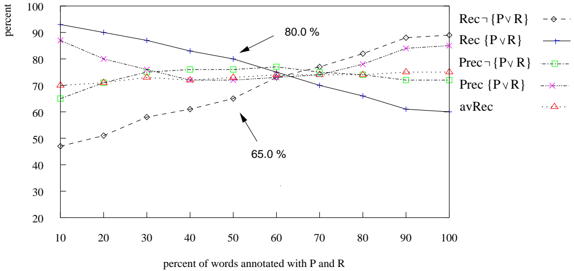
Figure 5: Combined classification of repetitions and prosody: 1365 \supset {P \vee R}, 1496 {P \vee R}, at the 50% threshold
