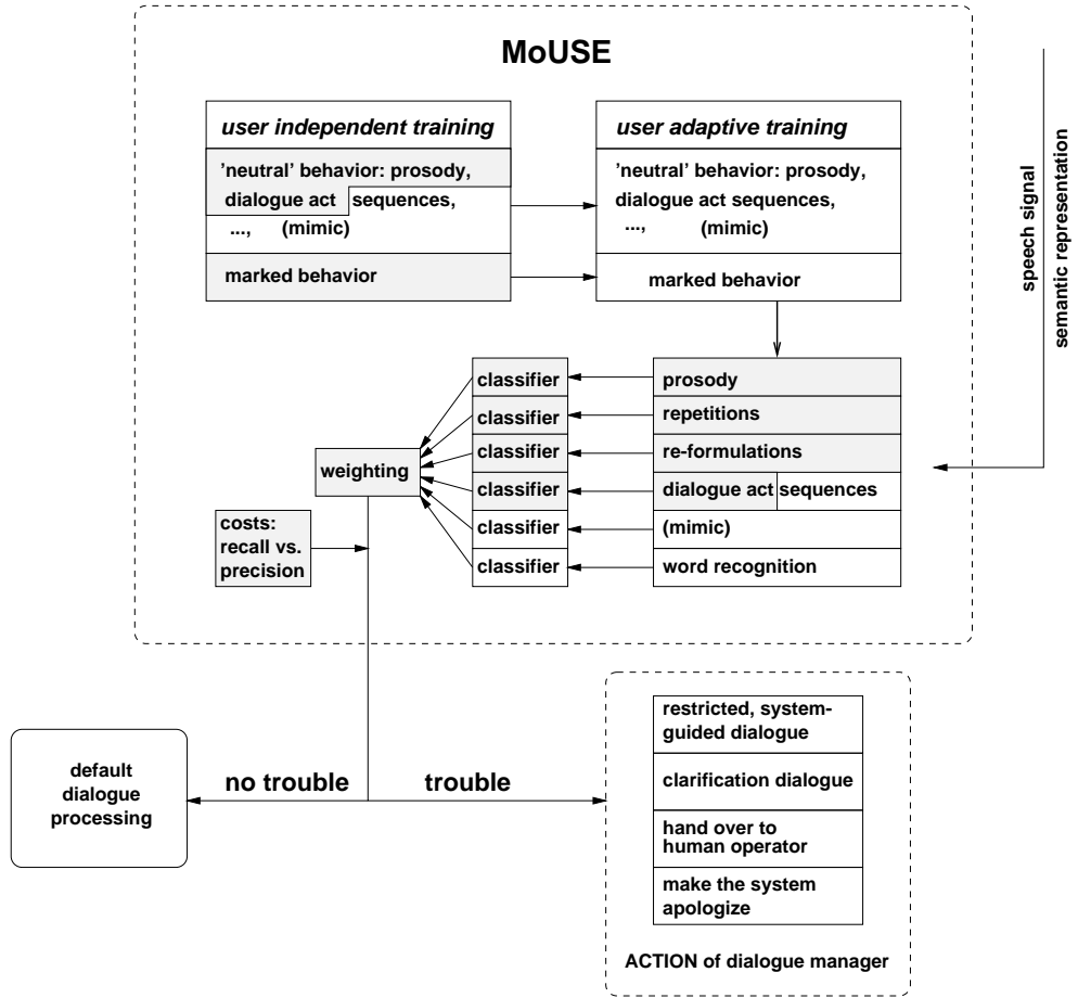
Figure 7: MoUSE: A Sketch of the Architecture; already implemented components are highlighted
