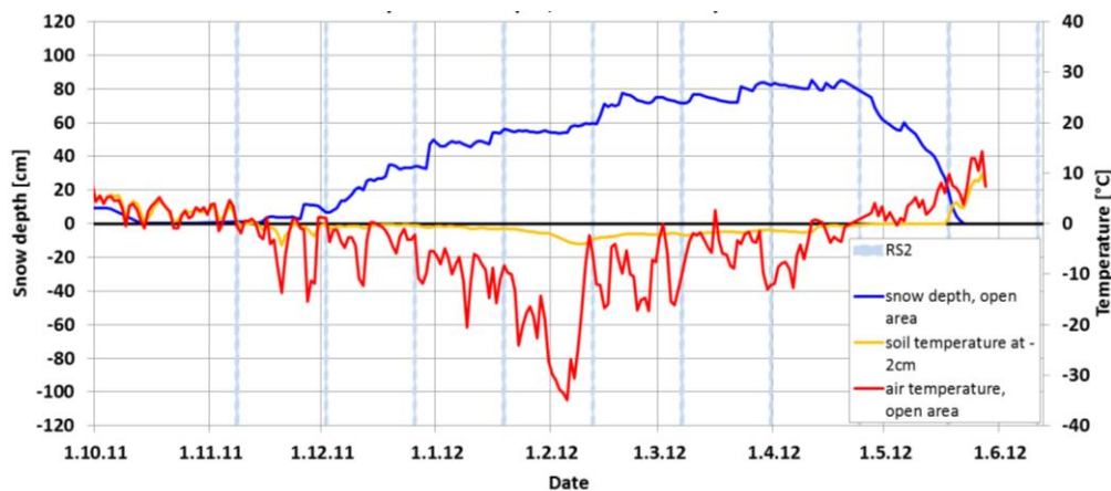
Figure 2. Snow depth (blue), air (red) and soil (orange) temperature curves recorded at the IOA measurement site (a forest clearing, where the ground vegetation consists of low lichen, moss and heather) for the entire winter period from snow accumulation starting in November 2011 until snow free periods in June 2012. The blue, vertical, dashed lines indicate the acquisition dates of RADARSAT-2: 8.11.11, 2.12.11, 26.12.11, 19.1.12, 12.2.12, 7.3.12, 31.3.12, 24.4.12, 18.5.12, 11.6.12 [19].
