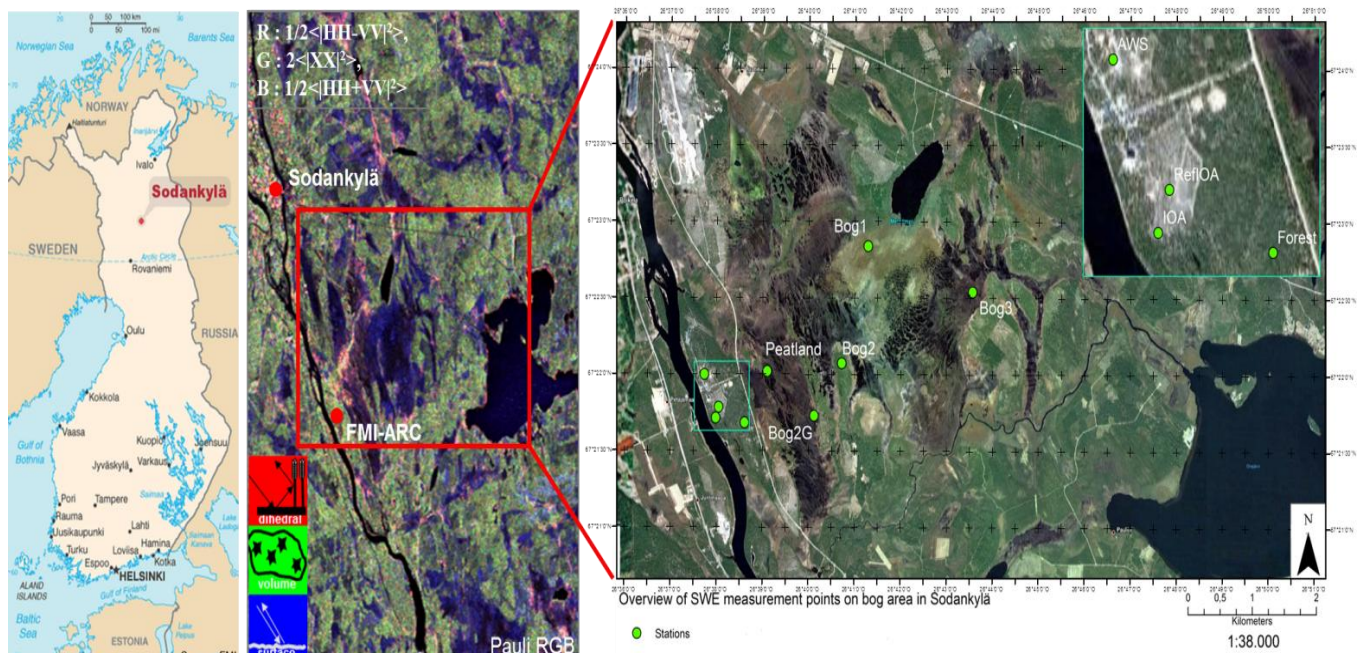
Figure 1. Test site location (red box) near the city of Sodankylä Finland, and C-band RGB image of a Pauli decomposition showing the surroundings of the test site (R: Double bounce scattering, G: Volume scattering, B: Surface soil scattering) as well as a zoom into a modified aerial image of the local measurement locations (green circles) around the FMI-ARC within the test site (AWS, IOA, RefIOA, Forest, Peatland, Bog1, Bog2, Bog2G, Bog3); SWE = Snow Water Equivalent [18].
