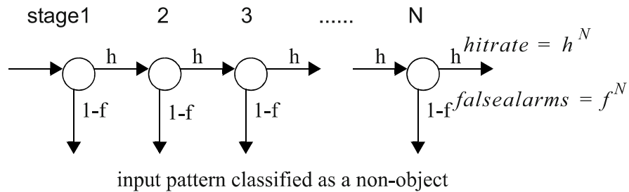
Fig. 4. Cascade of classifiers with N stages. At each stage a classifier is trained to achieve a hit rate of h and a false alarm rate of f .
