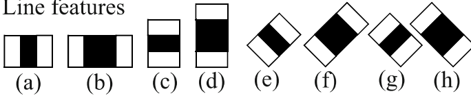
Fig. 2. Feature prototypes of simple haar-like and center-surround features. Black areas have negative and white areas positive weights.
