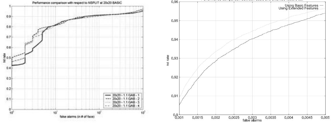
Fig. 7. Performance comparison with respect to (a) the order of the weak CART classifiers. GAB was used together with the basic feature set and a pattern size of 20x20. (b) Basic versus extended feature set: On average the false alarm rate of the face detector exploiting the extended feature set was about 10% better at the same hit rate (from [3]).
