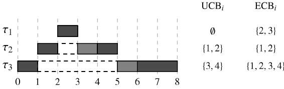
(b) Nested pre-emption: \tau_1 pre-empting \tau_2 pre-empting \tau_3 , causes higher costs than any non-nested pre-emption.
