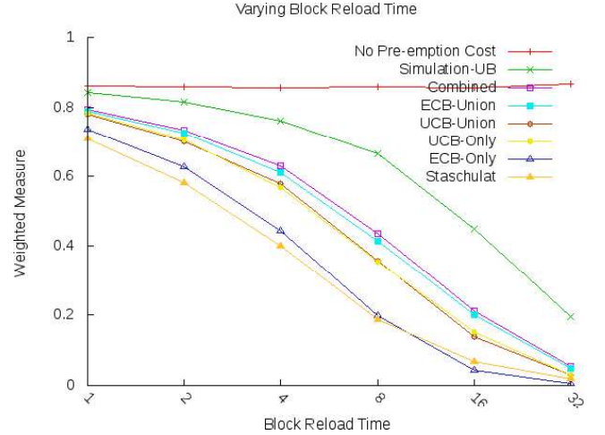
Fig. 12. Weighted schedulability measure; varying block reload time from 2^0 = 1\mu s to 2^4 = 32\mu s
