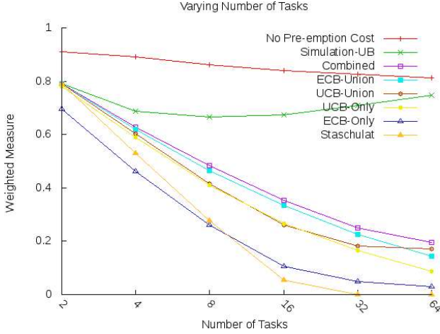
Fig. 10. Weighted schedulability measure; varying number of tasks from 2 = 2^1 to 2^6 = 64 .
