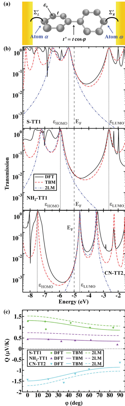
FIG. 4. (Color online) (a) Schematic of the TBM used to fit DFT-based transmission curves. (b) Transmission of M2 as a function of energy calculated with DFT, and the fits using the TBM and the 2LM. (c) Q as a function of \phi , comparing values obtained with the TBM and the 2LM to the DFT-based results. In panels (b) and (c), S-TT1, NH 2 -TT1, and CN-TT2 junction geometries were selected.
