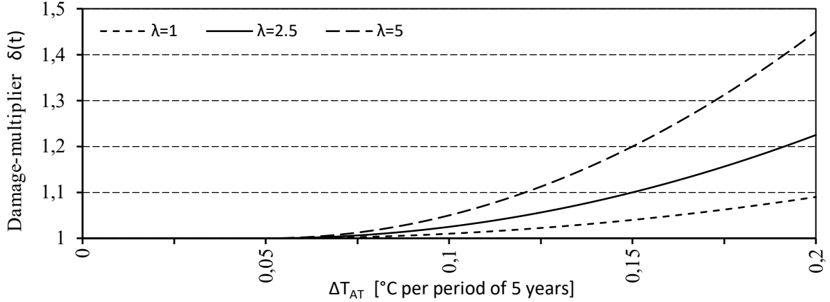
Figure 1. Shape of the damage-multiplier \delta(t) for an example with \nu=0.1 , \omega=2 and varying magnitudes of the parameter \lambda .
