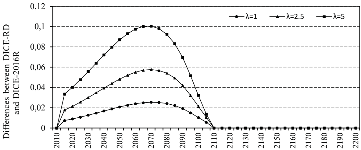
Figure 4. Optimal mitigation rates: Differences between DICE-RD and DICE-2016R for varying damage parameter \lambda (assuming \omega=2 and \nu=0.1 ).
