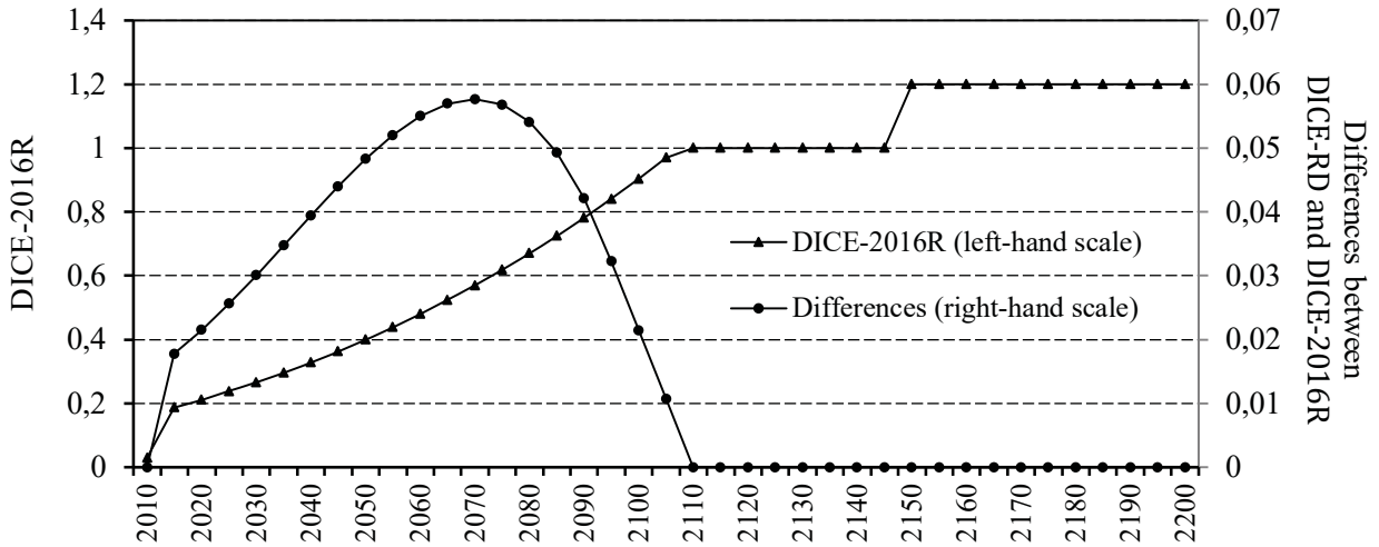
Figure 2. Optimal mitigation rates. Left-hand scale: DICE-2016R. Right-hand scale: Differences between DICE-RD and DICE2016R.
