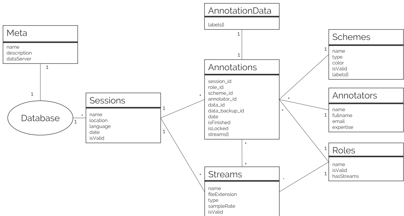
Fig. 11 Overview of NOVA’s database structure. Annotations and meta information on subjects, sessions, etc. are stored in different collections. NOVA includes necessary tools to maintain and populate a database
