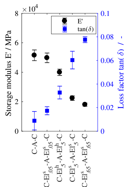
Figure 6. Storage module and loss factor for all specimens with CFRP on the outside at 20 °C and 1 Hz. Three specimens for each lay-up.
