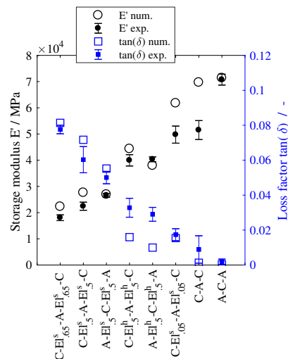
Figure 11. Comparison of experimental and numerical results for 20 °C and 1 Hz in ascending order of the experimentally determined storage modulus. Three specimens for each lay-up.
