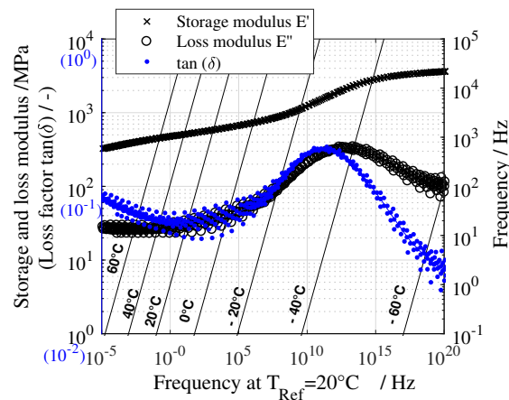
Figure 4. Master curve nomogram for tension DMA on the hard elastomer E'_{.5} .
