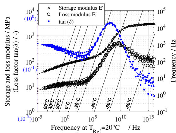
Figure 3. Master curve nomogram for tension DMA on the soft elastomer ( E'_{.05}, E'_{.5}, E'_{.65} ).
