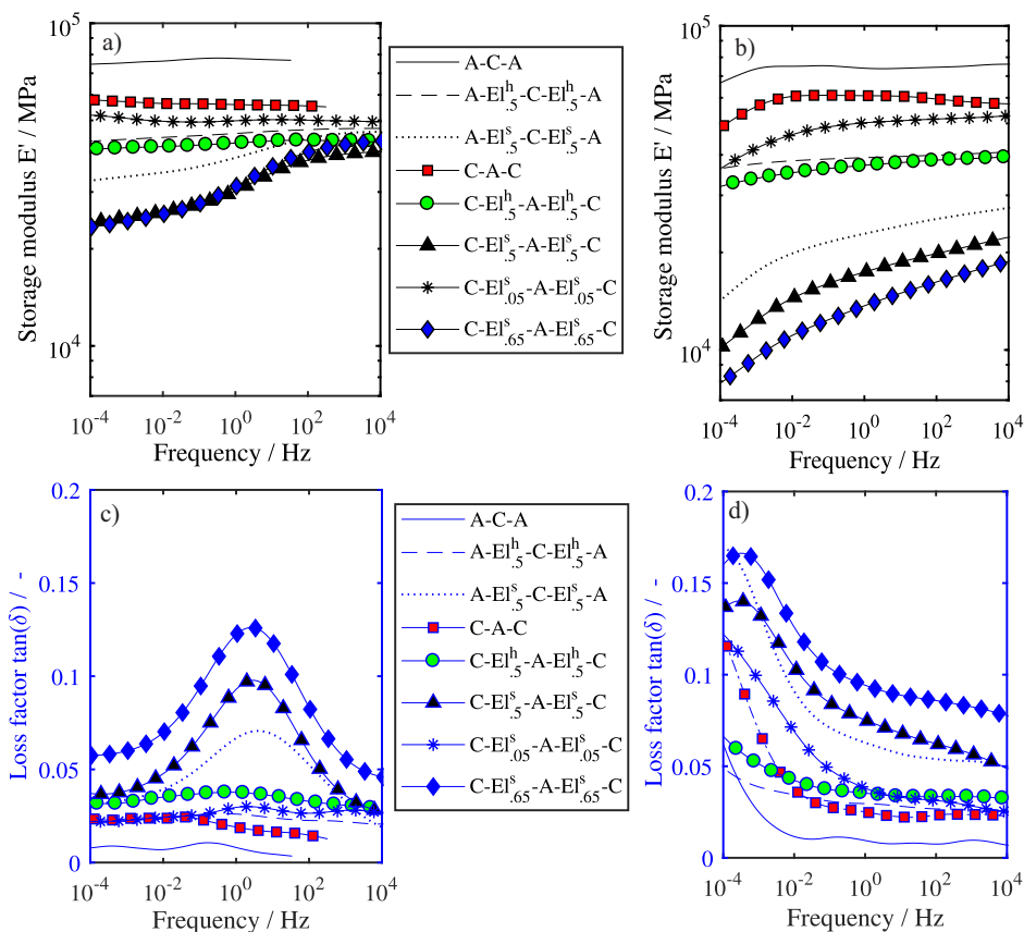
Figure 10. Master curves for all specimens at T_{\text{Ref}} = -40^{\circ}\text{C} (a,c) and T_{\text{Ref}} = 80^{\circ}\text{C} (b,d). For better visibility, fewer markers are displayed for the fitted curves.
