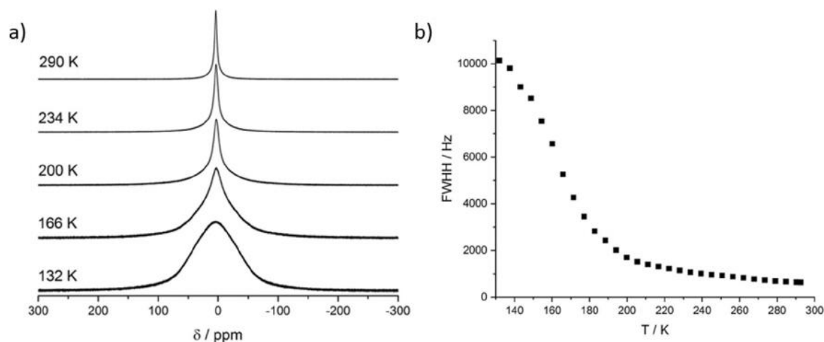
Figure 6. a) Temperature-dependent evolution of the ^7\text{Li} lineshape recorded in the temperature range from 132 to 290 K. b) Temperature-dependent linewidth of the ^7\text{Li} signal (full width at half height) recorded in the temperature range from 132 K to room temperature.
