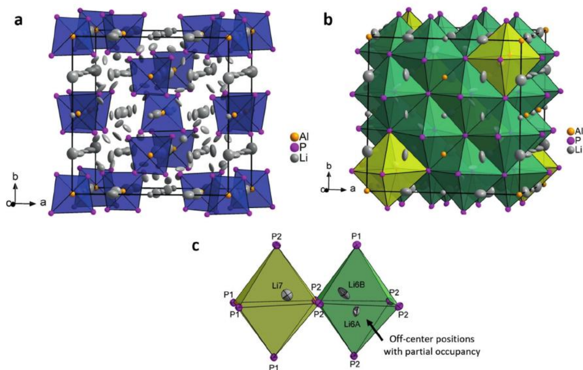
Figure 2. The crystal structure of \text{Li}_9\text{AlP}_4 as determined from experimental data. a) Unit cell of \text{Li}_9\text{AlP}_4 . The [\text{AlP}_4]^{3-} tetrahedra are highlighted in blue. \text{Li}^+ ions are located in tetrahedral and octahedral voids; some of them exhibit partial occupations (Table S3). b) Unit cell with emphasis on the two crystallographically independent octahedral voids: polyhedra of \text{Li6a/Li6b} and \text{Li7} are shown in green and yellow, respectively. c) Closeup of neighboring octahedral voids with partially occupied \text{Li6a} , \text{Li6b} , and \text{Li7} positions. Li, Al, and P are depicted in gray, orange, and purple, respectively (displacement ellipsoids set at 90% probability at 150 K).
