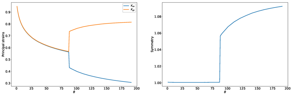
Fig. 3 Mean principal strains (left) and symmetry (right) of the minimiser as a function of \theta for the flat disk
