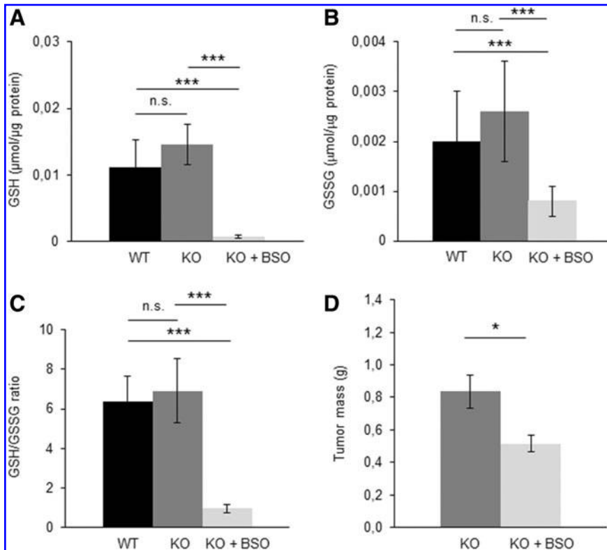
FIG. 3. Loss of Txnrd2 renders tumors susceptible to GSH depletion.
