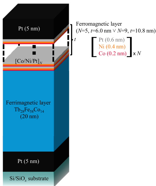
Figure 1. Schematic image illustrating the layer stacking of the two investigated FI/FM heterostructures.
