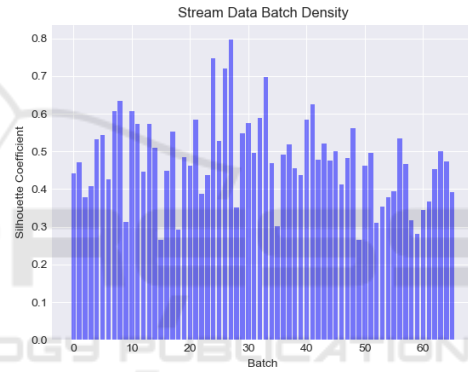
Figure 8: Silhouette coefficient values for clusters of batches 1 – 66.
