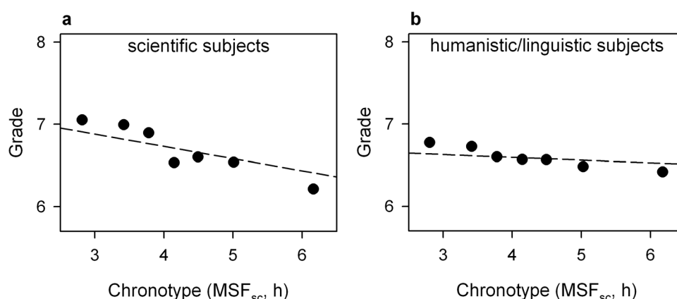
Figure 4. Influence of chronotype (MSF sc ) on grades by subject area. Data points represent mean grades with standard error of the mean (SEM). Since the SEM were very small, error bars are not always visible. Mean grades were calculated for 7 equal-sized groups of students based on chronotype (lower numbers corresponding to earlier chronotypes and higher numbers to later chronotypes, respectively). Regression lines representing the association between chronotype and grades (raw data) were calculated with multilevel mixed modelling separately per each subject. The raw data are shown in Supplementary Figure S3. The influence of chronotype on grades was significantly stronger for scientific subjects (biology, chemistry, physics, and mathematics) (a) compared with humanistic/linguistic subjects (Dutch, English, geography, and history) (b).
