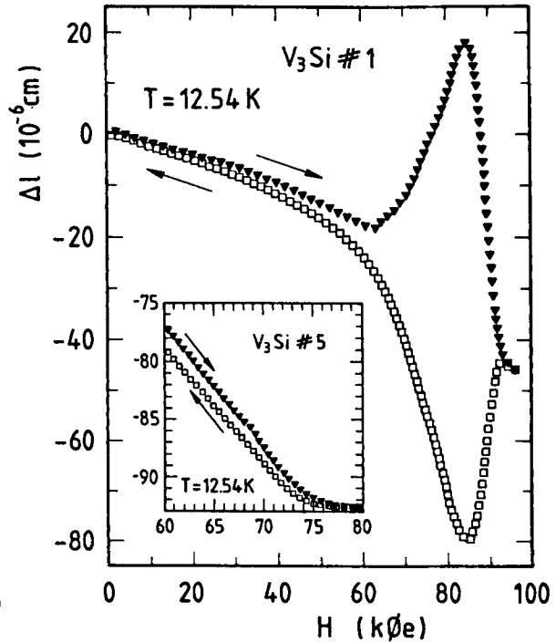
Fig. 6 Isothermal magnetostriction cycle, \Delta l vs H , measured at T=12.54 \text{ K} for \text{V}_3\text{Si} single crystal # 1. Inset shows high field data for very clean crystal # 5, showing a weak anomaly at H \approx 70 \text{ k}\phi\text{e} .
