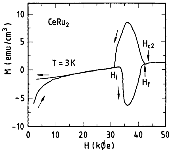
Fig. 1 Isothermal dc magnetization M vs H of \text{CeRu}_2 at T=3 K. Note that a Curie-Weiss contribution due to \geq 0.2 at% \text{Ce}^{3+} ions has to be subtracted from the data in order to obtain a constant susceptibility \chi_0 = (1.9 \pm 0.15) \cdot 10^{-5} \text{emu}/\text{cm}^3 , see text. Arrows indicate measurements done on raising and reducing the field, respectively, as well as onset ( H_i ), offset ( H_f ) fields of strong-pinning regime and the upper critical field ( H_{c2} ). In agreement with the magnetostriction results (Fig. 5), the magnetization is not strictly reversible below H=H_i .
