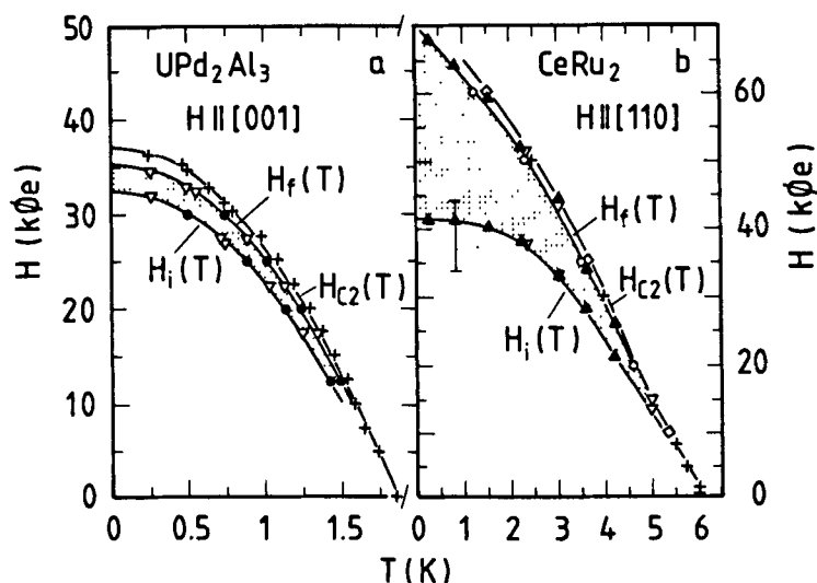
Fig. 2 H-T phase diagrams of UPd 2 Al 3 (a) and CeRu 2 (b). Anomalies in M(H,T) ( \nabla , Fig. 3), \Delta I(H) ( \blacktriangle , Fig. 5), \Delta I(T) ( \circ , Fig. 5) and \chi_{ac}(T) ( \bullet , Fig. 4) define onset [ H_i(T) ] and offset [ H_f(T) ] of irreversibilities, see text. Upper critical field H_{c2}(T) denoted by + [ \chi_{dc}(H,T) ] and [ \diamond coefficient of thermal expansion \alpha(T)=1/I \, dI/dT ].
