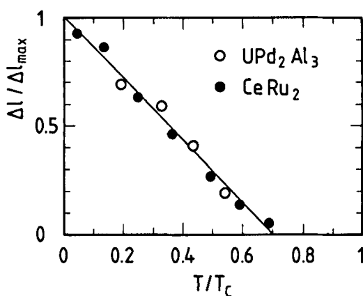
Fig. 7 Amplitude of magnetostriction anomalies vs reduced temperature CeRu 2 and UPd 2 Al 3 single crystals. Data have been normalized to coincide for T/T_c=0 .
