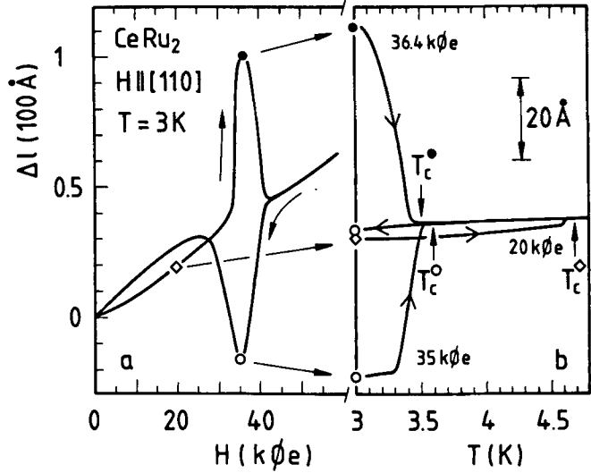
Fig. 5 \text{CeRu}_2 : Isothermal magnetostriction \Delta l vs H (a) and length change \Delta l vs T measured upon warming at different fields (b), starting from different points of the isothermal \Delta l(H) curve displayed in (a). \Delta l(T) data are shifted in order to coincide for the normal-state value. Field-cooled curve \Delta l(T) is shown for H=35 \text{ k}\phi\text{e} only.
