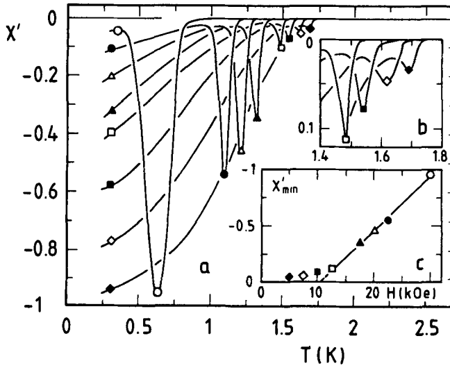
Fig. 4 Real part of \chi_{ac}(T, H=\text{const}) for \text{UPd}_2\text{Al}_3 (a, b) at different magnetic fields as indicated by the symbols (c) which mark the magnitude of the minimum vs the applied field.
