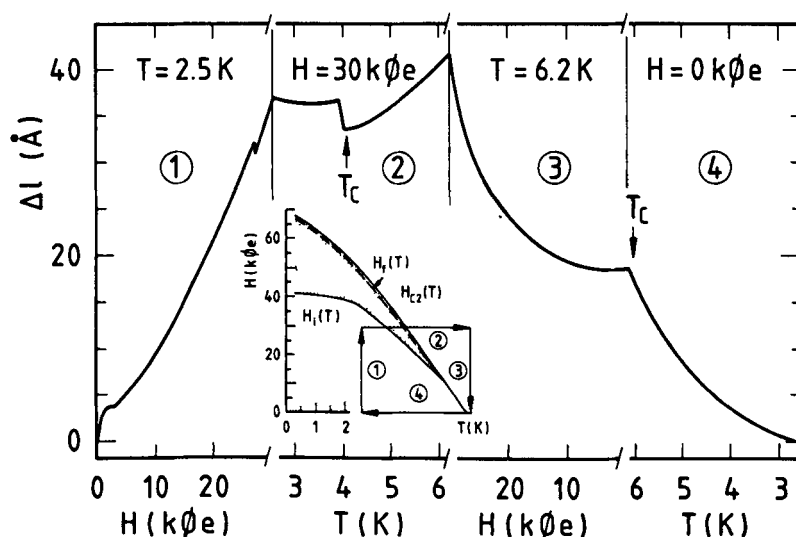
Fig. 8 Dilatometric investigation of a closed cycle in the H - T -plane of \text{CeRu}_2 (see inset) consisting of four subsequent measurements ( H \parallel [110] ): (1) isothermal magnetostriction ( T=2.5 K) starting from a superconducting state after zfc, (2) isofield thermal expansion ( H=30 kOe), (3) isothermal magnetostriction ( T=6.2 K) and (4) zero-field thermal expansion. Since the length balance is conserved, the small discontinuity in run (1) may be ascribed to a jump of flux bundles within the weak-pinning superconducting state. The characteristic length jump in run (2) occurs at T=(3.90 \pm 0.03) K, i.e. below T_c(30 \text{ kOe})=(3.98 \pm 0.02) K: both magnitude and sign of the anomaly depend strongly on the prehistory (1), cf. also Fig. 5.
