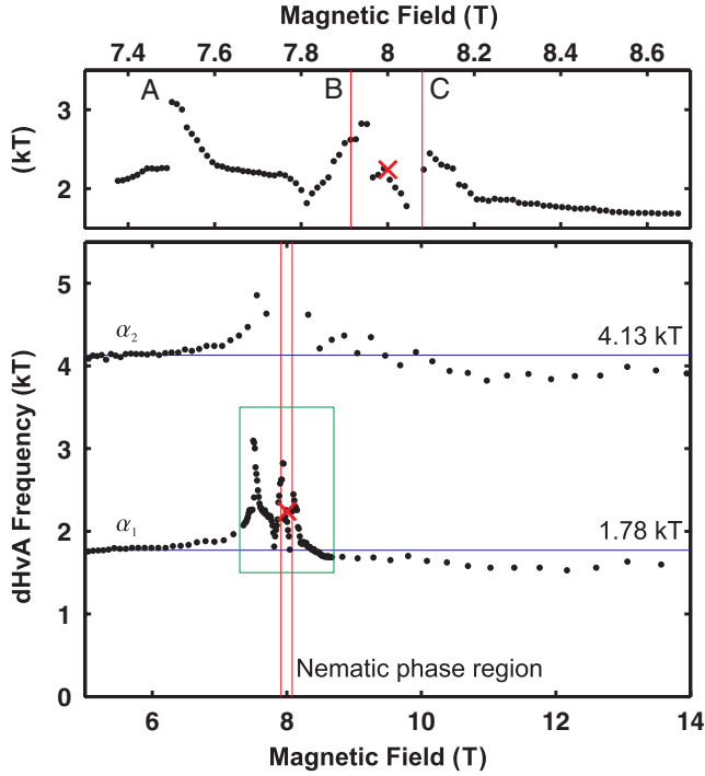
FIG. 3 (color online). Field dependence of the dHvA frequencies situated near 1.8 and 4.1 kT on the low-field side. These feature nonlinear changes in the metamagnetic region. The data points correspond to the location of peaks in Fourier transforms taken over field windows of equal inverse field width of 0.005 \text{ T}^{-1} . The field value for each data point corresponds to the inverse of the average inverse field. The lines mark the nematic phase field boundaries, and the cross the value of frequency measured inside the nematic phase. The top panel is a blowup of the data within the square in the bottom panel. Three peaks in F(B) , denoted A-C are observed near each of the metamagnetic features shown in Fig. 1. Corrections to field values due to the intrinsic magnetisation were found to be small.
