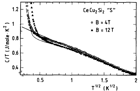
Fig. 3. Specific heat of the “S”-type \text{CeCu}_2\text{Si}_2 single crystal as C/T versus T^{1/2} for various fields applied parallel to the a -axis. Dotted ( B = 4 \text{ T} ) and thin solid ( B = 12 \text{ T} ) lines represent the data after subtraction of a nuclear contribution (see text). The thick solid line represents the dependence C/T = \gamma - \alpha T^{1/2} .
