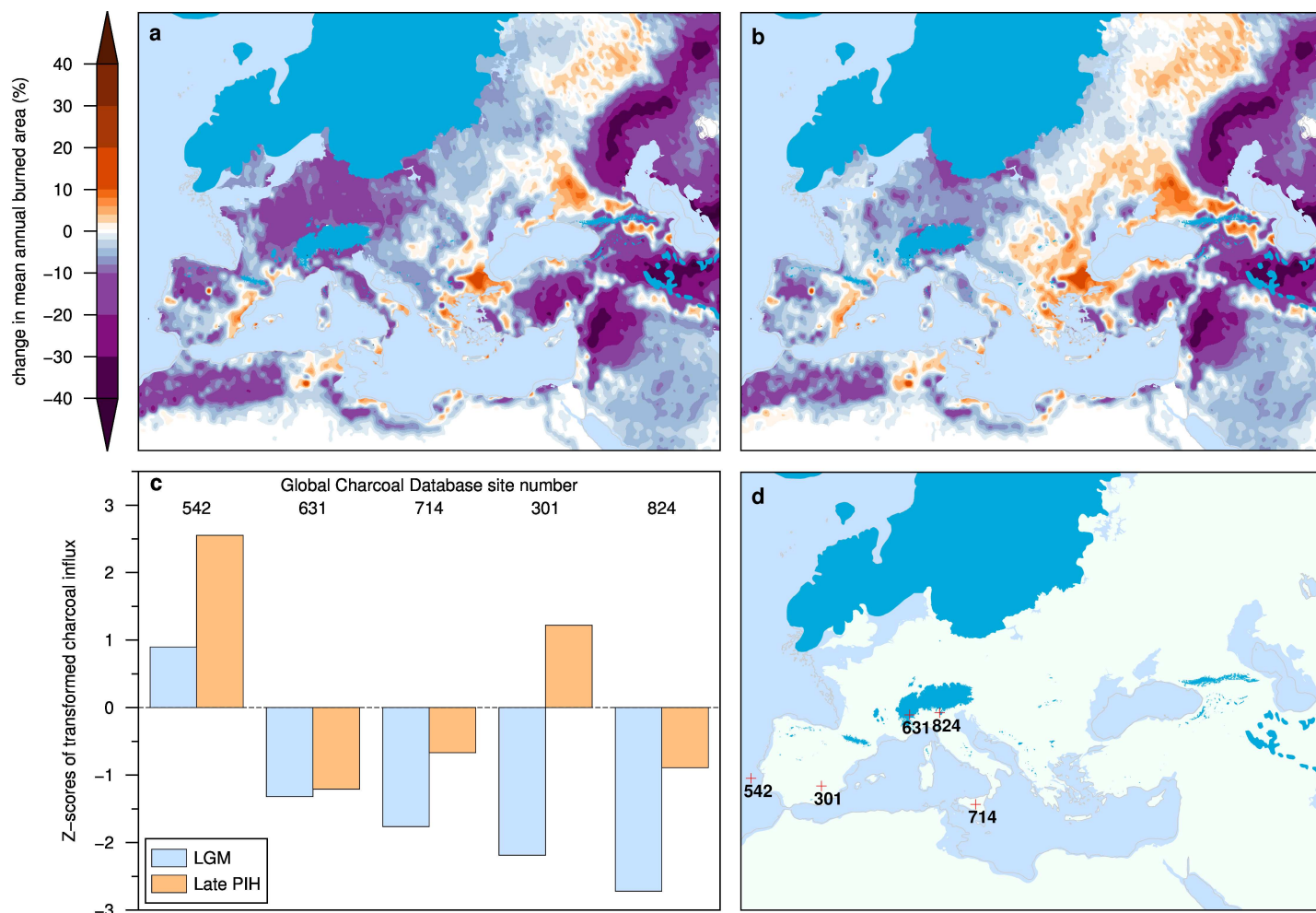
Fig 5. Change in burned area fraction between LGM and the Preindustrial Holocene (PIH). Difference in mean annual burned area fraction between LGM and the late PIH (AD 1770) in (A) the LPJ ensemble mean simulation without human burning, and in (B) the LPJ ensemble mean scenario including human burning. Panel (C) shows relative charcoal accumulation at the LGM and late PIH (AD 1650±200 yr) at the five Global Charcoal Database sites (D) containing lake and marine sediment microcharcoal dating to LGM [23]. The Z-scores of transformed charcoal influx are calculated relative to the preindustrial Holocene base period (0.2–12 ka) following [21]. At all charcoal sites the charcoal influx is smaller in samples dated to LGM compared to the PIH. The gray outline is the LGM coastline.
