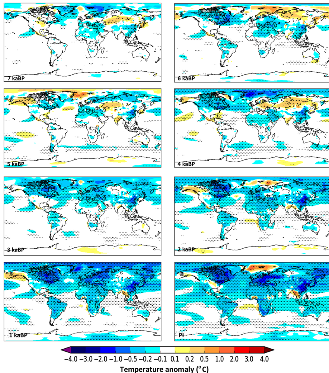
Figure 3. DJF temperature anomalies (°C) for KK10 minus control at time slices from the late pre-industrial period (1850 CE) to 7 ka BP. The stippling indicates grid boxes where the anomalies are significant at the 95 % level using Wilcoxon rank sum statistical analysis.
