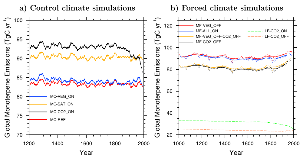
Figure 2. (a) Time evolution of the mean global monoterpene emissions in the control climate simulations: 1 (MC-REF) (red), 2 (MC-SAT_ON) (yellow), 3 (MC-VEG_ON) (blue), and 5 (MC-CO2_ON) (black). The series represent smooth, mean decadal monthly values. (b) Time evolution of the mean global monoterpene emissions in the forced simulations: 6 (MF-VEG_OFF) (red), 7 (MF-ALL_ON) (blue), 8 (MF-VEG_OFF-CO2_OFF) (yellow), 9 (MF-CO2_OFF) (black), 10 (LF-CO2_OFF) (orange), and 11 (LF-CO2_ON) (green). MEGAN solid series represent smooth, mean centennial monthly values, and MEGAN dotted series represent smooth, mean decadal monthly values. LPJ-GUESS series have 100 year resolution from 1000 to 1700, 20 year resolution from 1700 to 1900, and 10 year resolution from 1900 to 2000. See Table 5 for a description of the different simulations.
