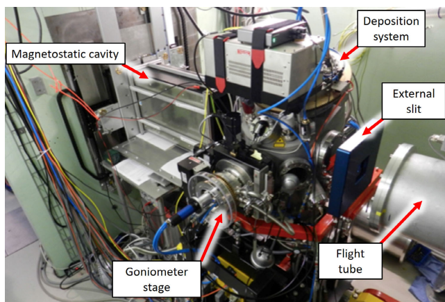
Figure 5. Sputter deposition system, integrated into the REFSANS beamline. A magnetostatic cavity for NSF is installed between the neutron optics (hidden from view behind the green wall to the left of the photograph) and the in situ deposition system. Details of the goniometer stage with encoder and details of the external slit system are visible, which is located before the entrance window of the evacuated flight tube.
