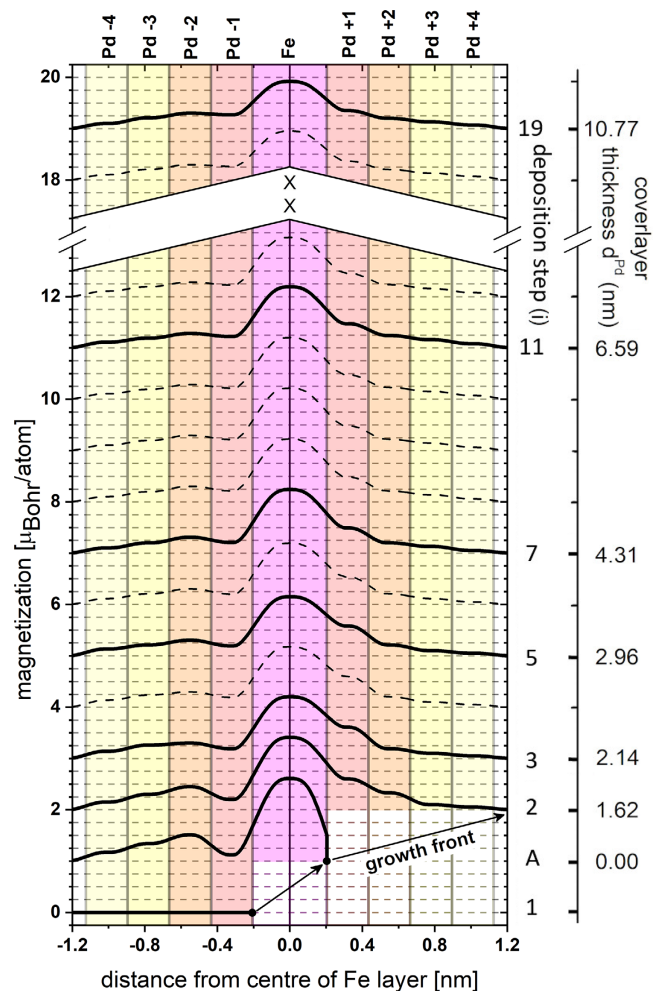
Figure 8. Magnetization profiles of an in situ grown Pd/Fe/Pd trilayer as a function of deposition step i = 2 –19 of the covering Pd layer, and distance from the center of the Fe layer, obtained from in situ PNR ( i = 1 denotes the deposition step of the initial Pd layer, i = A is the deposition step, in which the Fe layer was grown). For reasons of clarity, dashed lines show interpolated curves. They are displayed vertically shifted by 1 \mu_{\text{B}} \text{atom}^{-1} . The regions of induced magnetization in the Pd—denoted as Pd–4, Pd–3, Pd–2, Pd–1 (Pd seed layer) and Pd+1, Pd+2, Pd+3 and Pd+4 (Pd capping layer)—extend up to 0.92 nm to either side of the Fe layer, with the remaining Pd being regarded as nonmagnetic. Although in the initial stages of Pd capping layer growth a strong asymmetry of the magnetization of Pd–1 and Pd+1 is observed, the asymmetry vanishes as the structural symmetry of the Pd/Fe/Pd trilayer is restored. This is accompanied by a slight reduction in the magnetization of the Fe layer.
