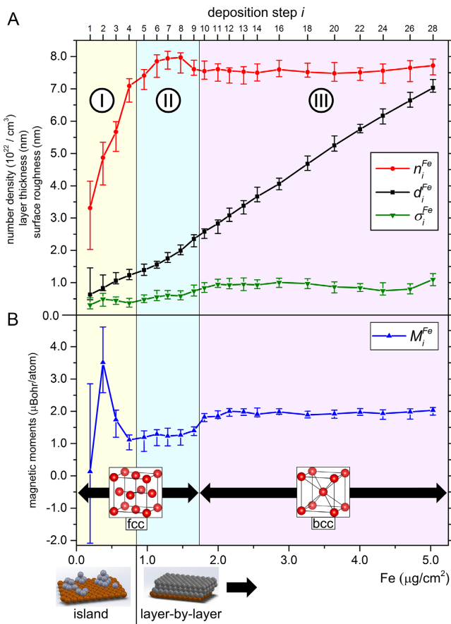
Figure 7. The fit parameters of the epitaxially grown Fe layer as a function of deposition step i . Three main regimes (I–III) with different characteristic behaviors for the number density n_i^{\text{Fe}} , thickness d_i^{\text{Fe}} , interfacial roughness \sigma_i^{\text{Fe}} , and magnetization M_i^{\text{Fe}} can be identified. Shown are also the concluded growth modes (island/layer-by-layer) and crystalline structures (fcc/bcc). Reproduced with permission. [59] Copyright 2017, American Physical Society.
