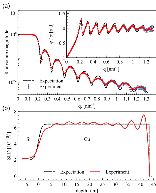
Figure 9. a) The reconstructed reflection R = |R|e^{i\phi} of the Cu/Si substrate sample, using the reflectivity data shown in Figure 6. The inset shows the phase information of the reflection. b) Scattering length density of the reconstructed sample, using the reflection shown in the top graph. The depth at 0 nm refers to the Cu/Si interface. “Expectation” represents the reflection and SLD as obtained from traditional fitting.
