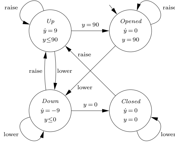
Figure 9. Gate automaton
