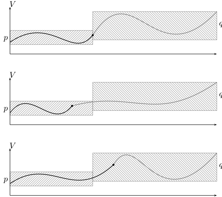
Figure 6. Composed trajectories satisfying \Box p \cdot \Box q
