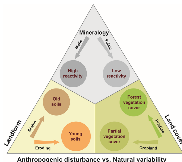
Figure 1. Factorial design of project TropSOC studying biogeochemical cycles in Central African tropical forest and agricultural landscapes in relation to mineralogy, landform, and land cover types.
