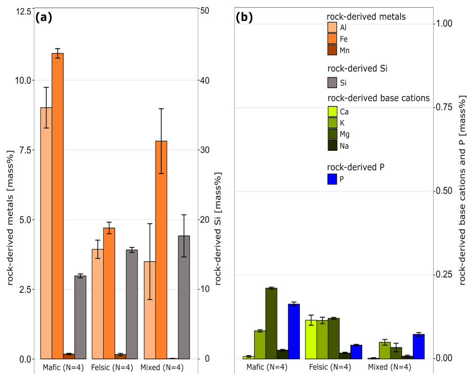
Figure 4. Soil chemical composition of subsoil in stable, old-growth closed-canopy forests (no erosion) in the three investigated geochemical regions (mean \pm standard error). The data illustrate the convergence of elemental concentrations between the three regions as a result of weathering and soil development. Abbreviations explained in Fig. 3. Note the difference in scale on the y axis between panels (a) and (b).
